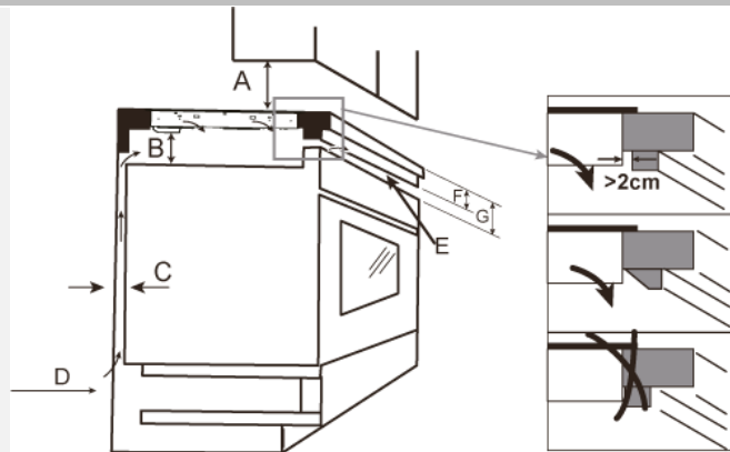
Graph I: Installation distances B1= with and without heat source
