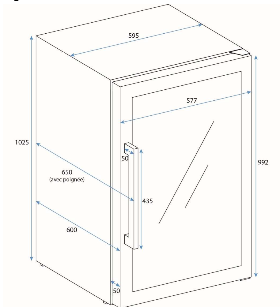
Figure :Cotation
