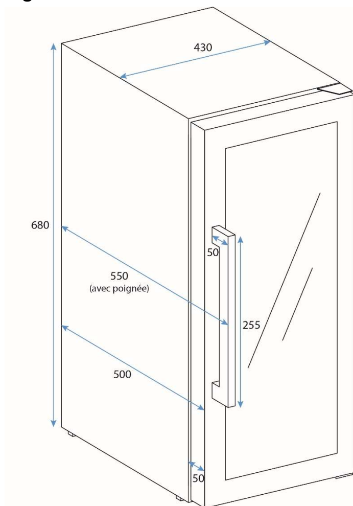
Figure :Cotation
