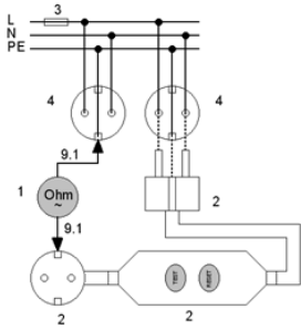
Picture 1a: Protective conductor resistance measurement
