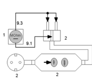
Picture 2a: Insulation resistance measurement Input
