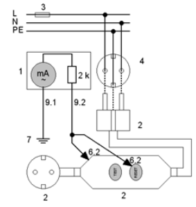
Picture 4a: Contact current measurement
