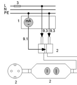
Picture 3a: Direct protective conductor current measurement
