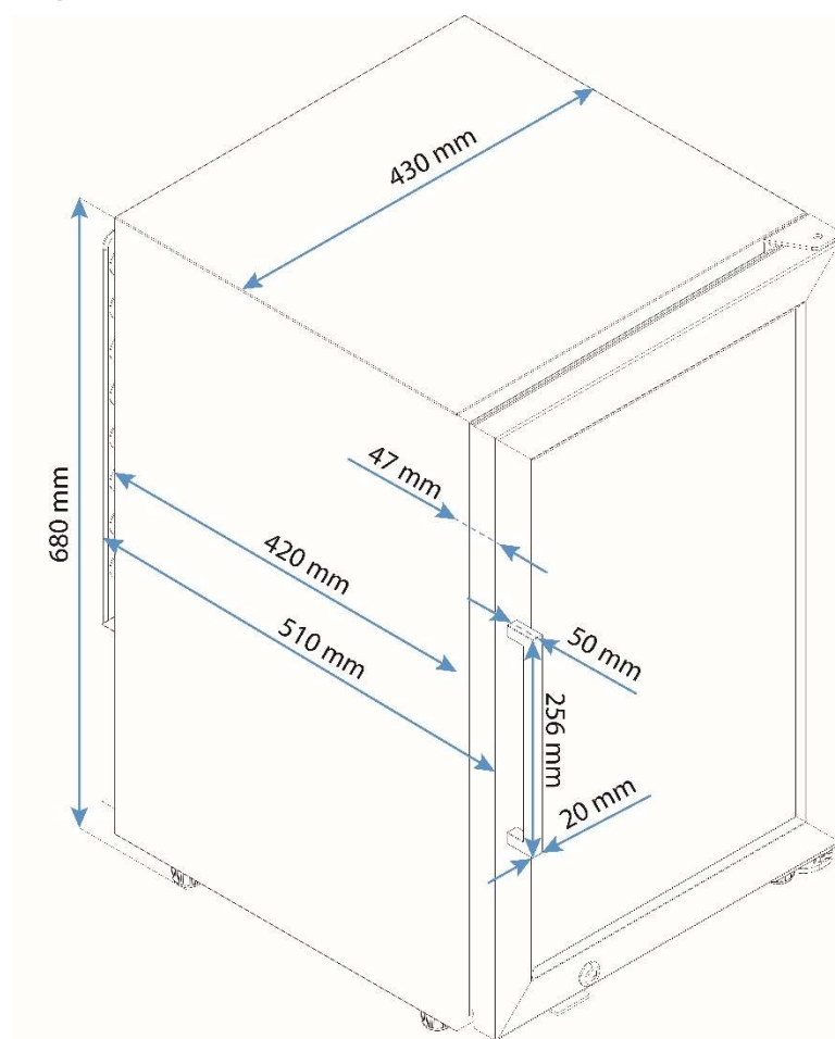
Figure :Cotation
